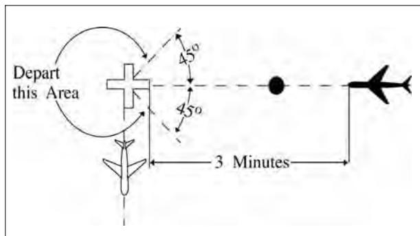
FIG 6-3-1 Separation Minima
