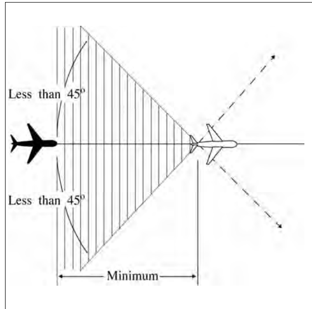
FIG 8-3-1 Same Courses
