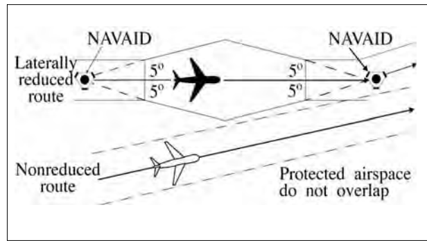
FIG 8-4-2 Separation Methods
