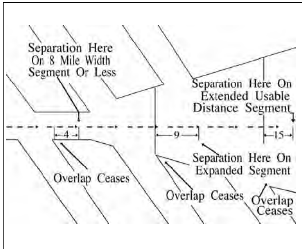
FIG 6-5-7 RNAV Minima
